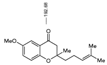
^{13}\text{C} NMR (126 MHz, \text{CDCl}_3 )
